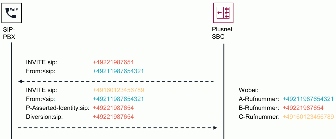
Abbildung 5: Call Forwarding
